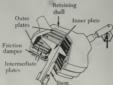
Pedestal-type dynafocal subassembly.
